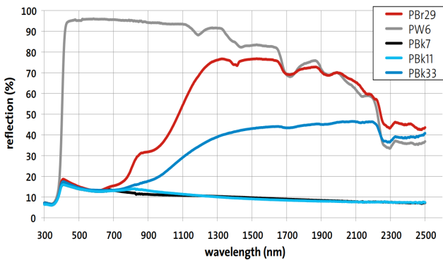
Figure 2: Reflection curves of different pigments
